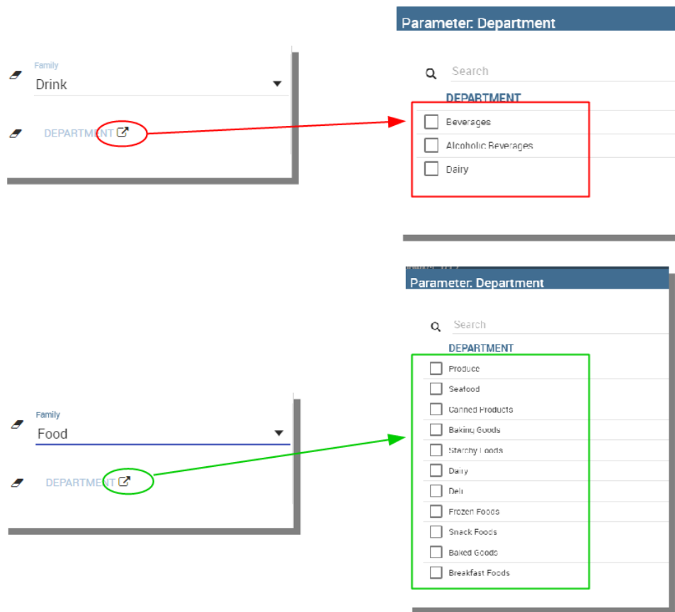
Fig. 5.248: Filtering with correlation.
