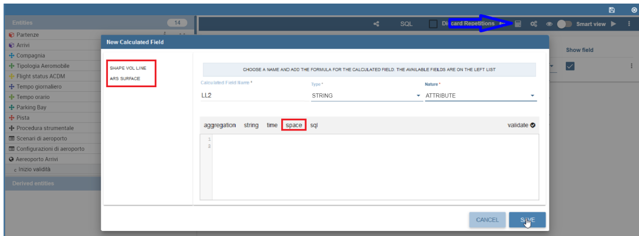
Fig. 5.222: Calculated field wizard with spatial filters.
