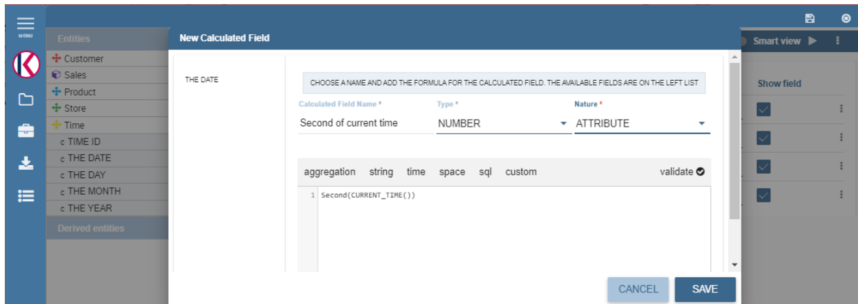
Fig. 5.231: Creating calculated field with function second(date).
