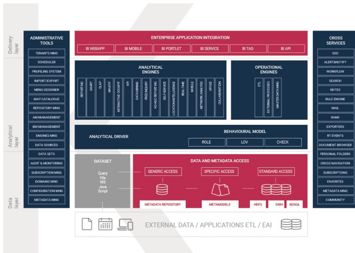
Fig. 3.3: Knowage Server architecture detail.
