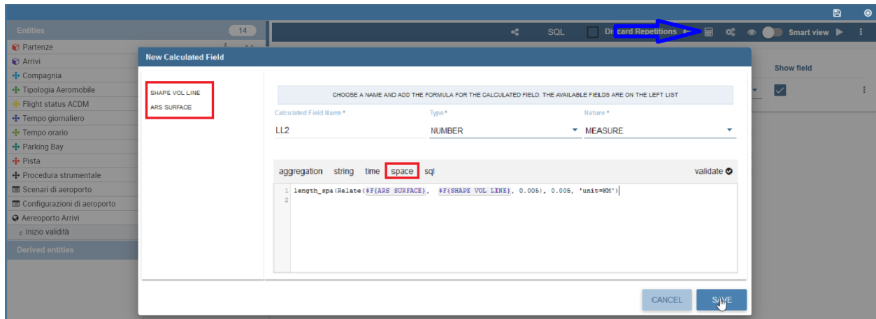
Fig. 5.225: Example of added calculated field using a spatial function.
