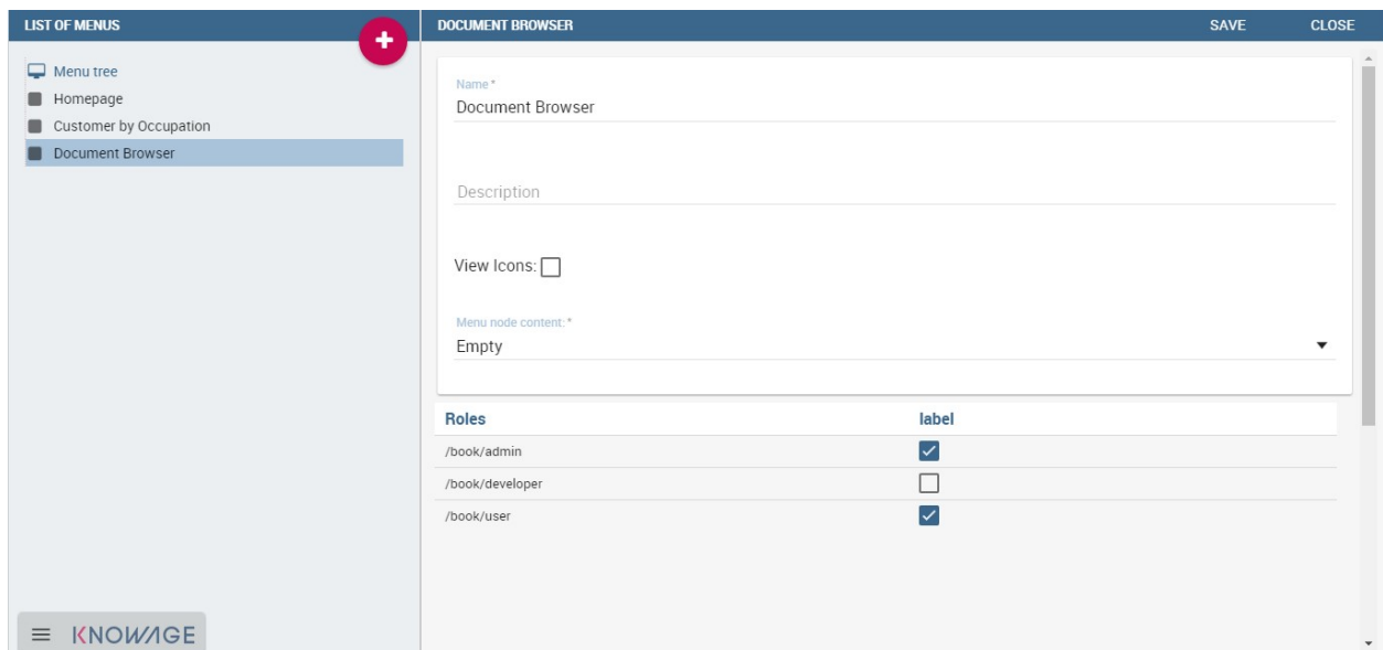
Fig. 3.15: Menu tree actions.
