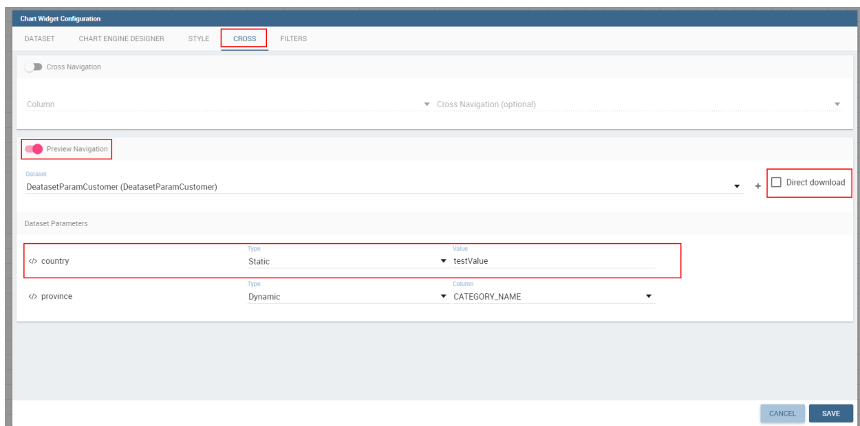
Fig. 5.526: Preview navigation configuration.
