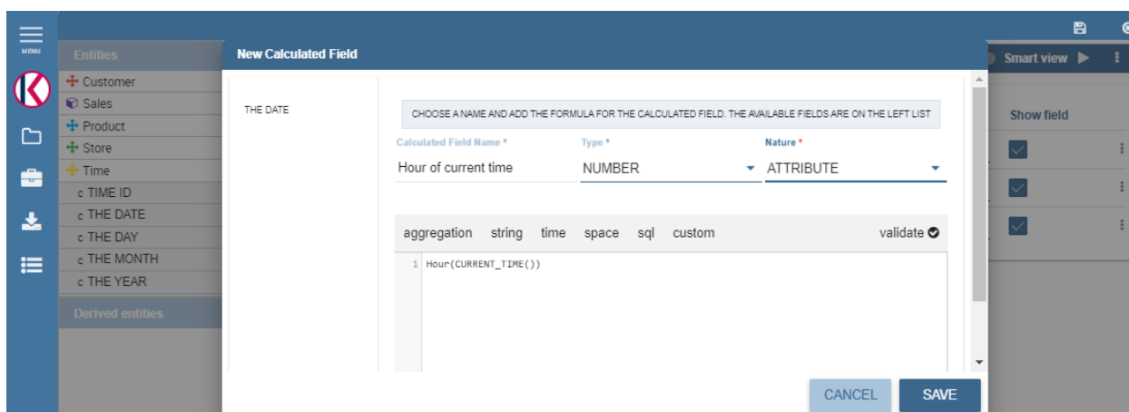
Fig. 5.230: Creating calculated field with function hour(date).
