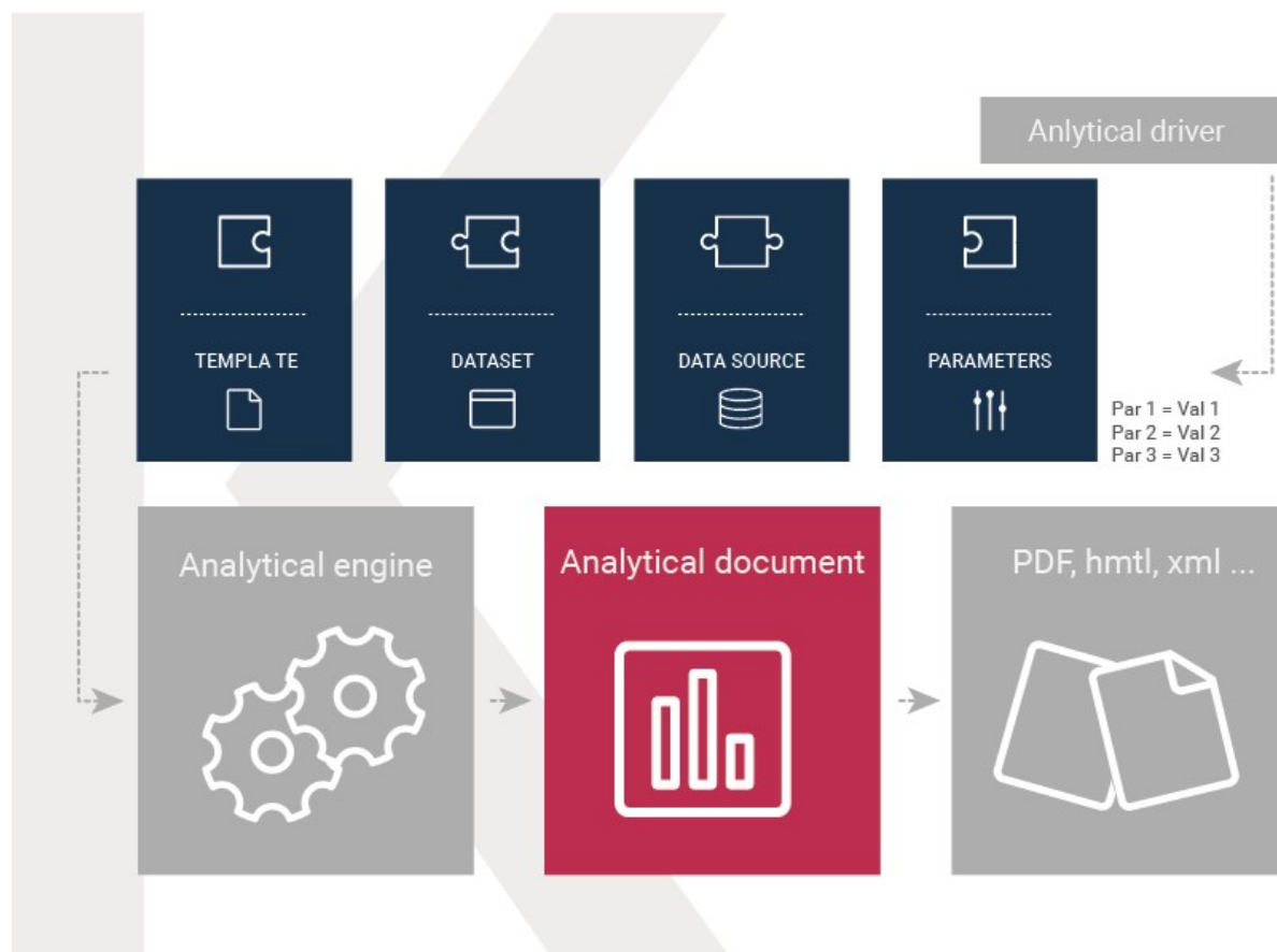
Fig. 5.50: Components of Knowage analytical document.
