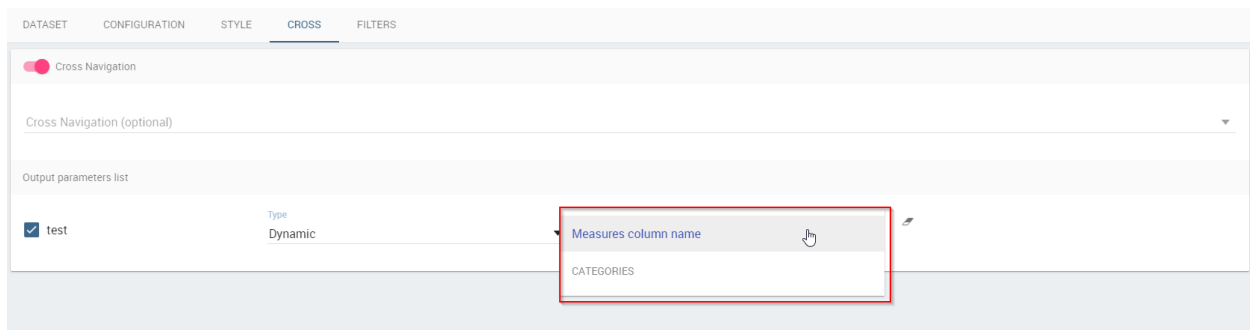
Fig. 5.163: Cross navigation for cross table widget.
