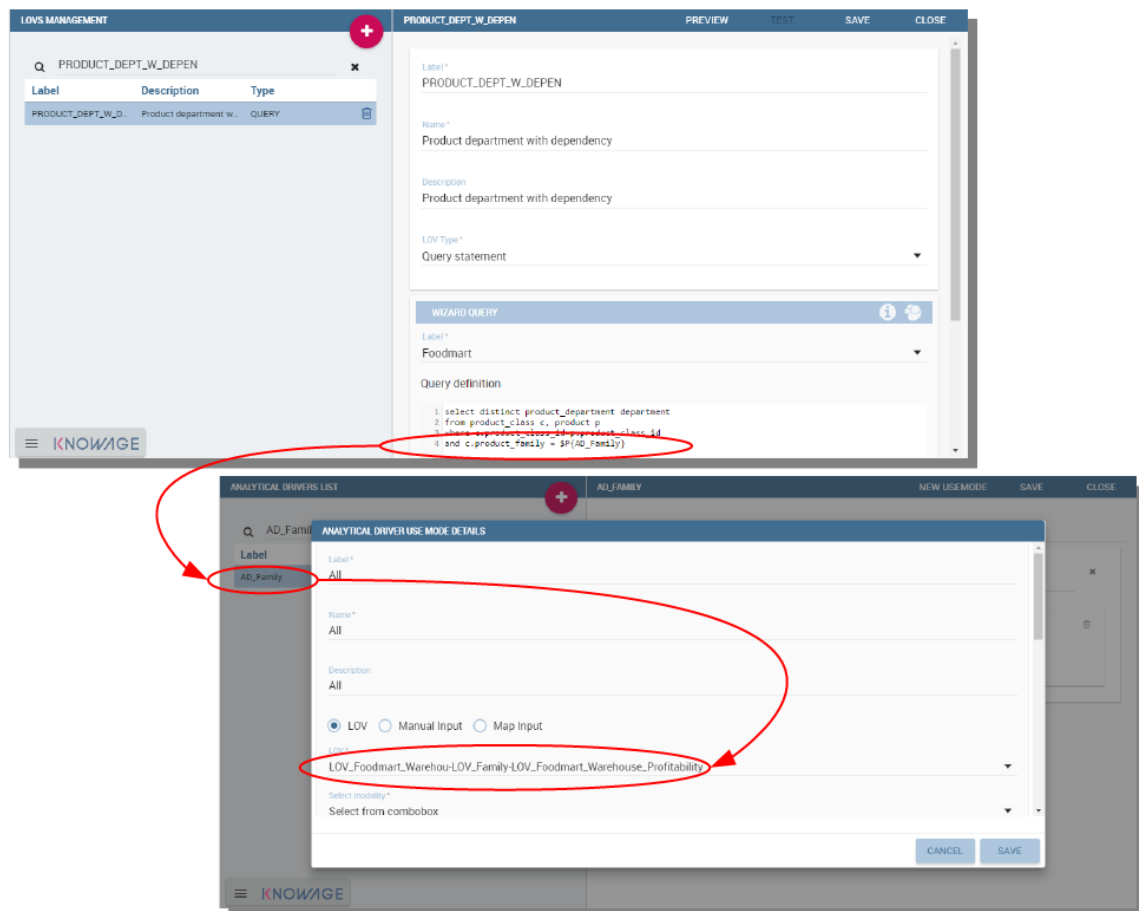
Fig. 5.68: Correlation passing driver values to LOV query .
