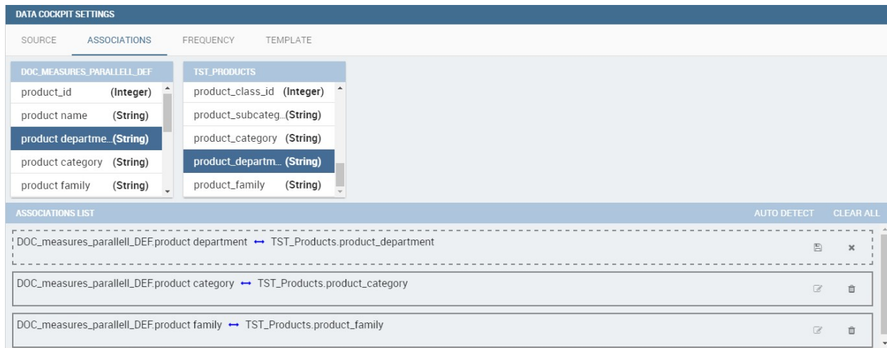
Fig. 5.193: Associations between dataset columns.
